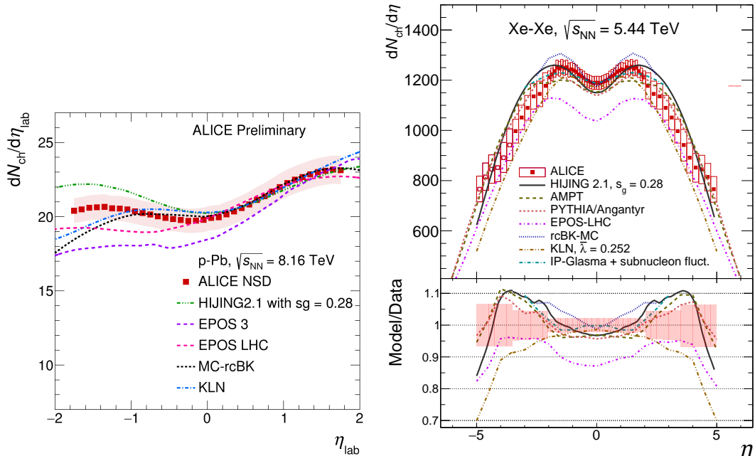
(a) dN_{\text{ch}}/d\eta in p–Pb collisions
