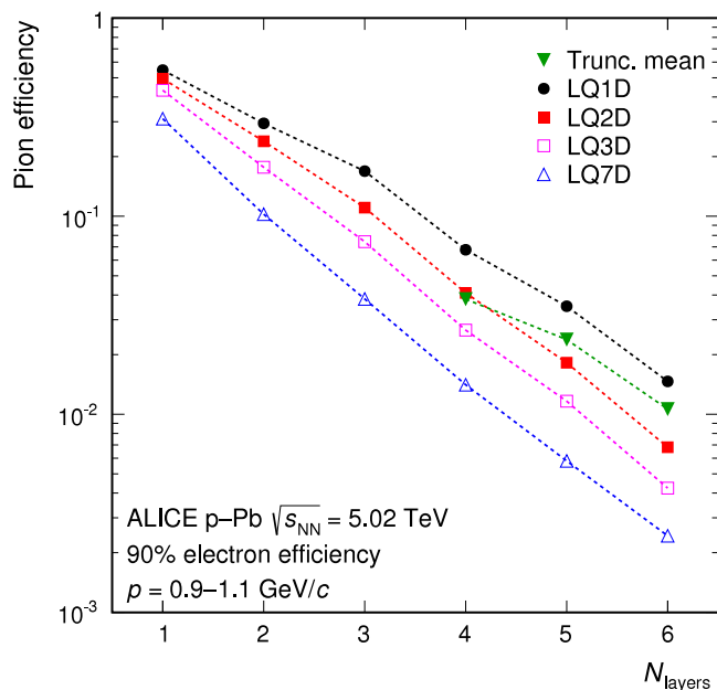
Fig. 42. Pion efficiency as a function of electron efficiency (top, for 6 detector layers) and as a function of the number of detector layers (bottom, for 90% electron efficiency) for the various eID methods. The results are compared for the momentum interval 0.9–1.1 GeV/c in p–Pb collisions at \sqrt{s_{NN}} = 5.02 TeV. The results of the truncated mean method are only shown for a minimum of 4 tracklets, where the resolution is better than 18% (see Fig. 39).
