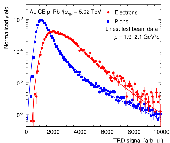
Fig. 36. Total integrated charge, normalised to the tracklet length, measured in a single read-out chamber for electrons and pions in p–Pb collisions at \sqrt{s_{NN}} = 5.02 TeV, in comparison with results from test beam measurements (solid lines) [47,105]. The electrons and pions from test beam measurements were scaled by one common factor to compensate the difference in gain of the two data sets.
