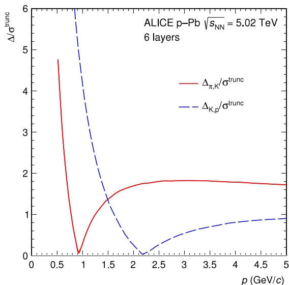
Fig. 40. Measured separation power ( \frac{\Delta}{\sigma^{trunc}} = \frac{\sigma_{\pi,K}^{trunc} - \sigma_{K,\pi}^{trunc}}{\sigma^{trunc}} ) for \pi/K and K/p separation as a function of momentum.
