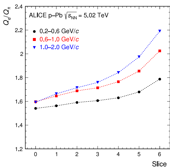
Fig. 41. Ratio of the average signal of electrons to that of pions as a function of the depth in the detector (slice number; the lowest (highest) slice number is farthest away from (closest to) the radiator).
