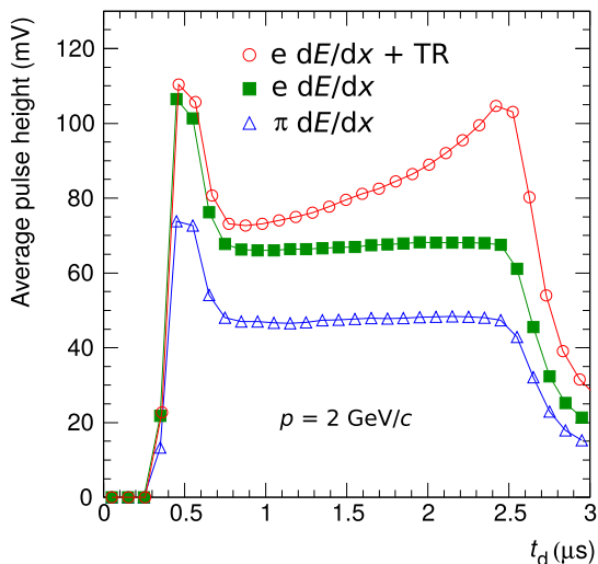
Fig. 5. Average pulse height as a function of drift time for pions and electrons (with and without radiator). The time axis is shown with an arbitrary offset of 0.3\ \mu\text{s} . The measurements were performed at the CERN PS with prototype read-out chambers that were smaller in overall size (active area 25\ \text{cm} \times 32\ \text{cm} ) but otherwise similar in construction to that of the final detector. Figure taken from [47].
