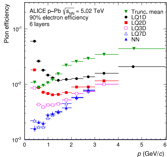
Fig. 43. Pion efficiency (for 90% electron efficiency) as a function of momentum for the truncated mean, LQ1D, LQ2D, LQ3D, LQ7D and NN methods. The results are from p–Pb collisions at \sqrt{s_{NN}} = 5.02 TeV and for tracks with signals in six layers.
