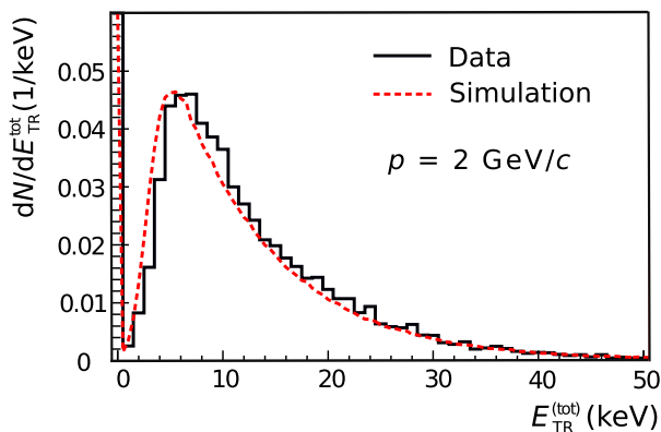
Fig. 8. Measured and simulated spectra of TR produced by electrons with a momentum of 2 GeV/c for the ALICE TRD sandwich radiator. Figure adapted from [52].
