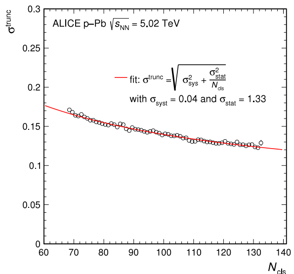
Fig. 39. Resolution of the truncated mean signal as a function of the number of clusters in p-Pb collisions at \sqrt{s_{\text{NN}}} = 5.02 \text{ TeV} .
